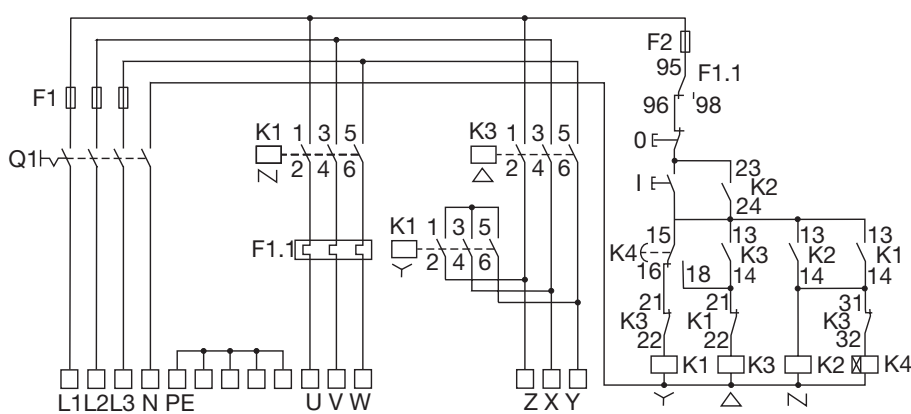
Star-delta starter
