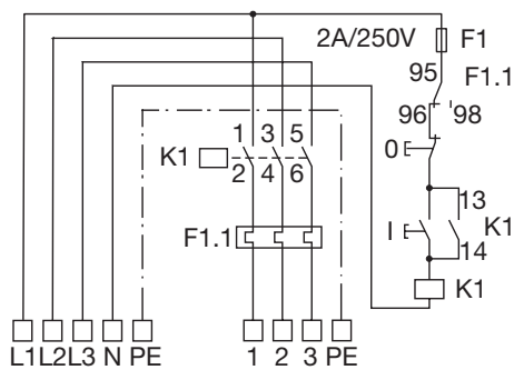
Direct circuit
